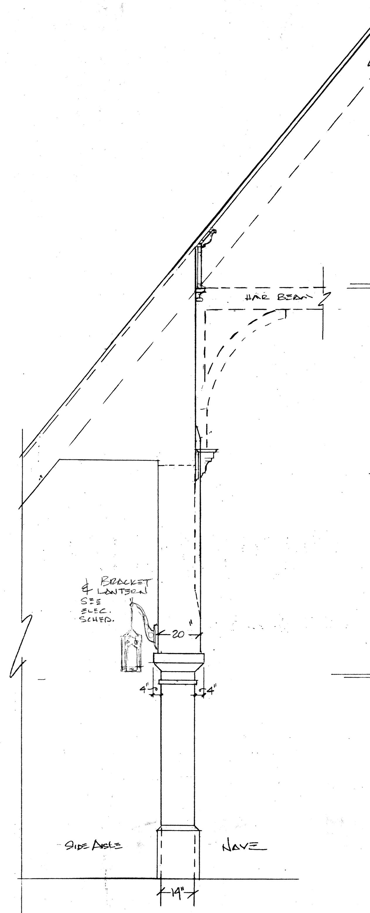
HAMMER BEAM BAND SAWN CORBELS SCALE: 2" = 1'0" (WITH APPLIED TOP & BACK PLATES) PRODUCT #915 / MOULDING CENTER, NO. HOLLYWOOD EACH CORBEL CONSISTS OF 2-5/8" CORBELS JOINED BACK & TOP PLATES W/ 3/4" GROOVE IS APPLIED
